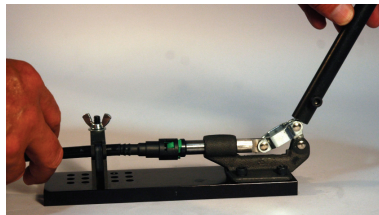
No. AFP-2000 Fuel Line Assembly Tool
